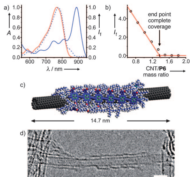
Figure 2. a) Vis/NIR absorption spectra of P6 (red line), P6 -CNT (blue line), and excitation spectrum of P6 -CNT at 1020 nm (blue dashed line) all in THF; b) P6 emission at 930 nm with increasing concentration of CNT. The arrow marks the point where all porphyrin is bound to CNT. [ P6 ] = 2.1 mg L -1 ; c) molecular mechanics 19 optimized structure of 3 × P6 ·(8,6) CNT based on the calculated mass ratio; d) HRTEM image of P6 -CNT (scale bar 2 nm).
